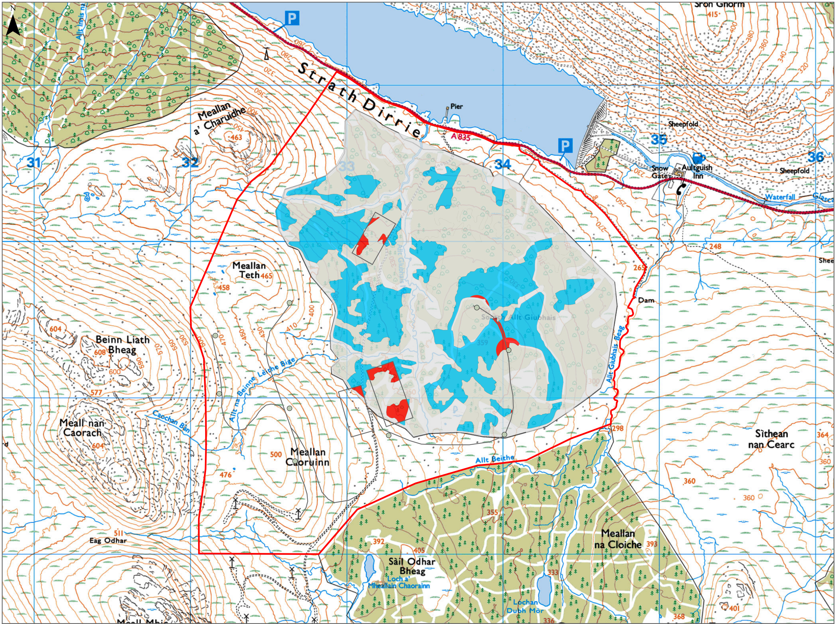
Figure 16.2: Felling Plan
